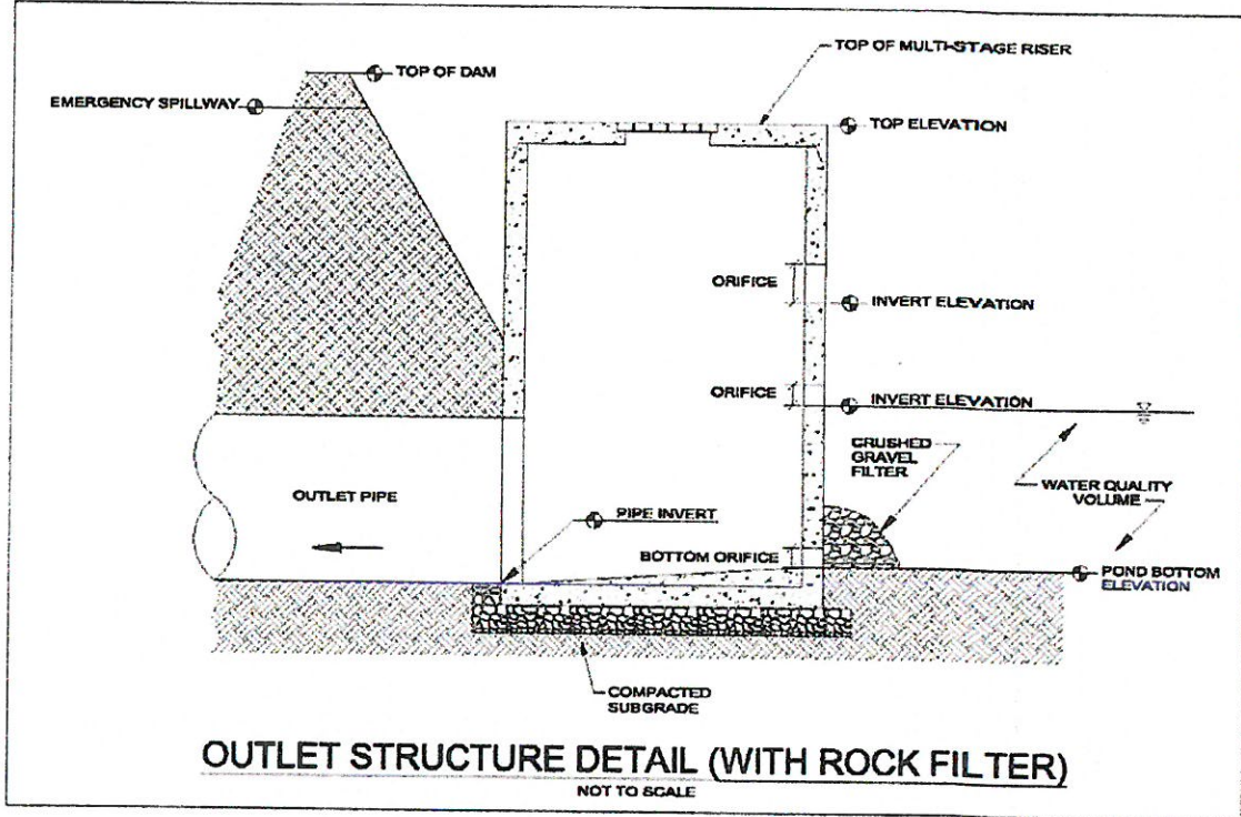
Figure 4 – Detention Pond Outlet Structure Examples
